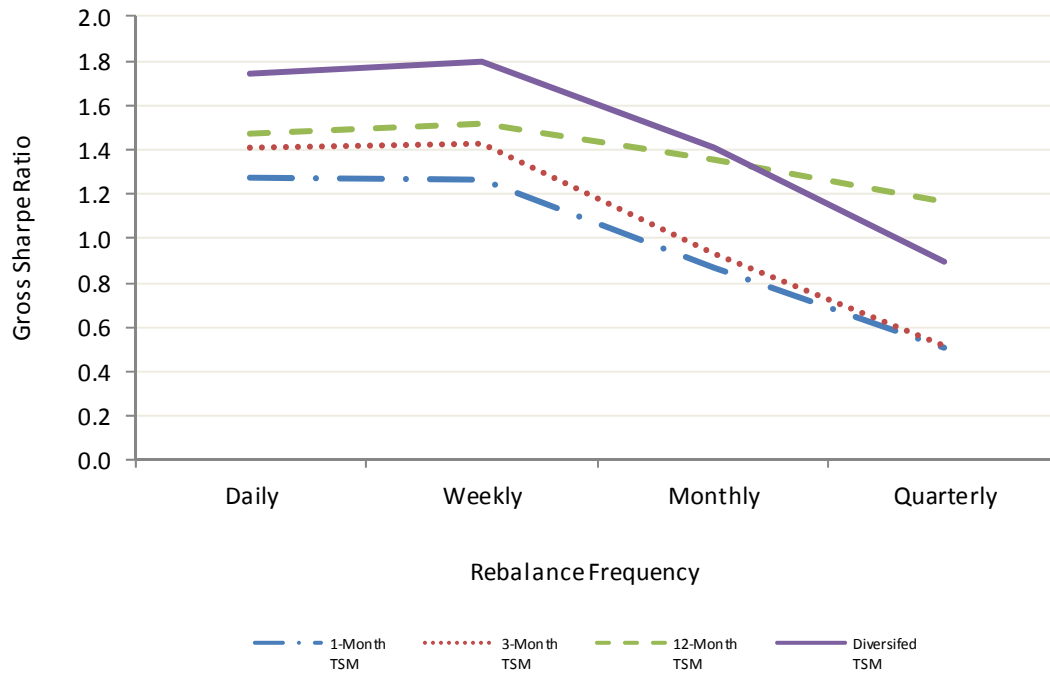
Figure 6. Gross Sharpe Ratios at Different Rebalance Frequencies. This figure shows the Sharpe ratios gross of transaction costs of the 1-month, 3-month, 12-month, and diversified time series momentum strategies as a function of the rebalancing frequency.
